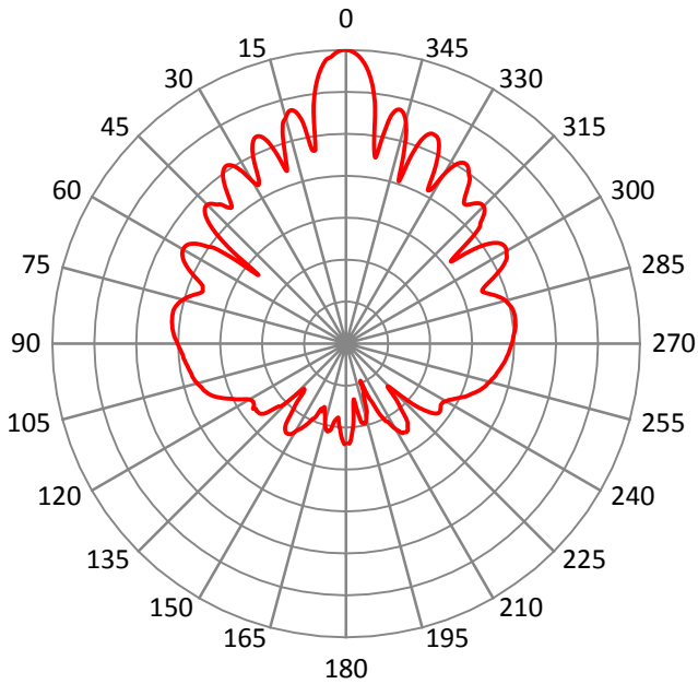
Azimuth @ 5.8GHz
