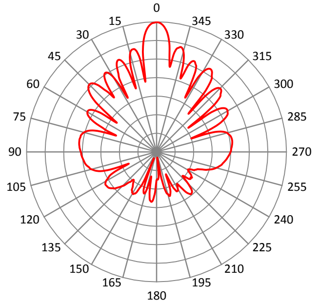
Elevation @ 5.8GHz
